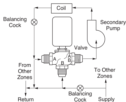
Figure-5 Typical Primary-Secondary Piping.
