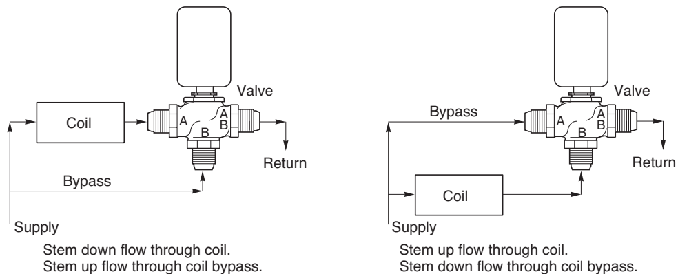
Figure-3 Typical Piping for Control of Heating or Cooling Coil.
