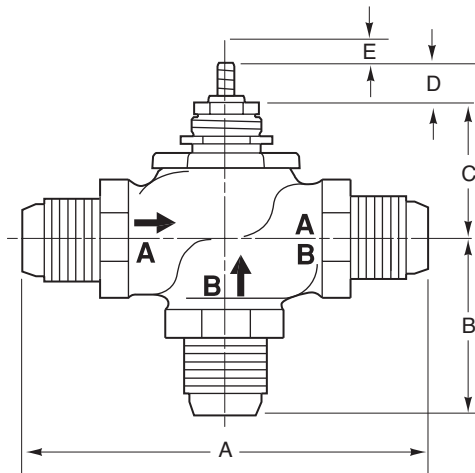
Figure-6 Dimensions for VB-7312 Series Valve Bodies.
