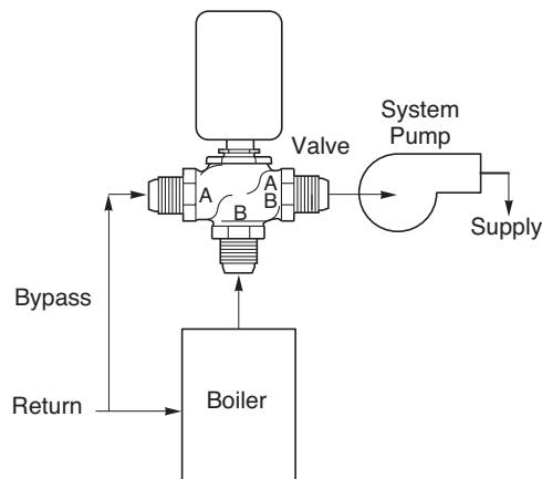
Figure-4 Typical Boiler Piping When Used in a Hot Water Reset Application.
