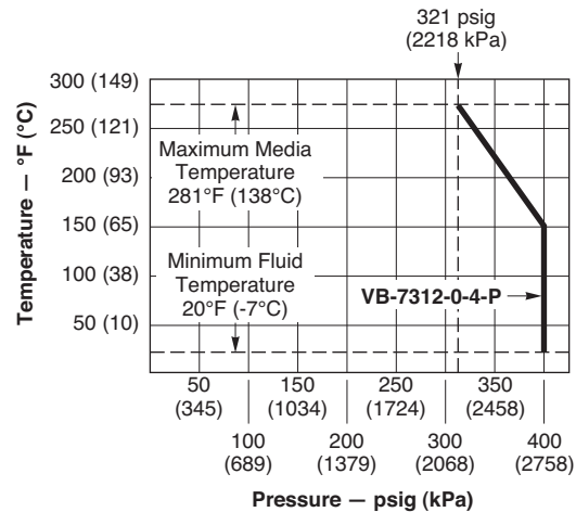
Figure-2 Temperature and Pressure Ratings for VB-7312 Series Valve Bodies.
